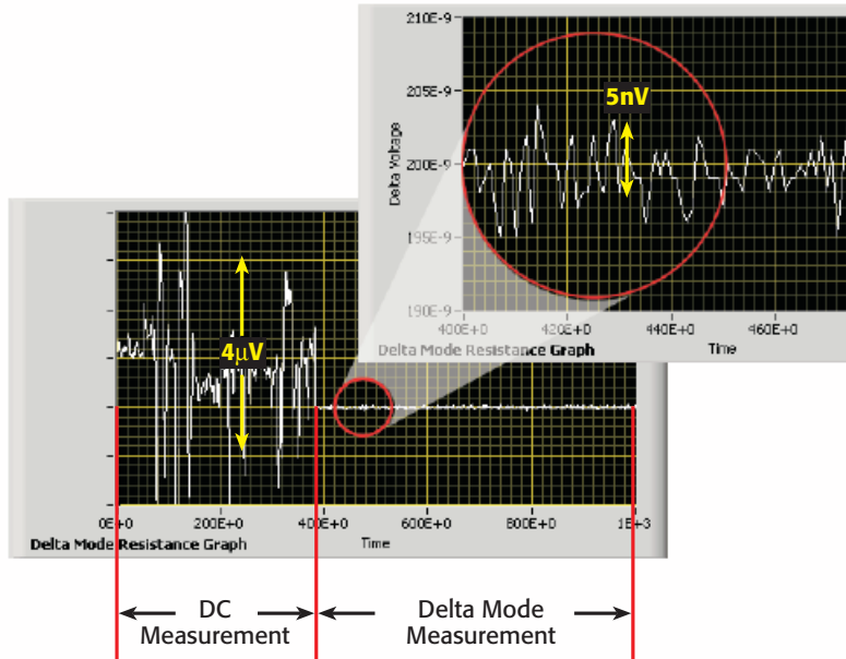
Figure 2. Delta mode offers 1000-to-1 noise reduction.
